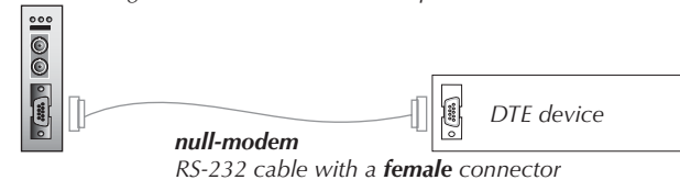
J-RS232-TF-01 or J-RS232-TF-01(SC) (DTE configuration with a male RS-232 port)
